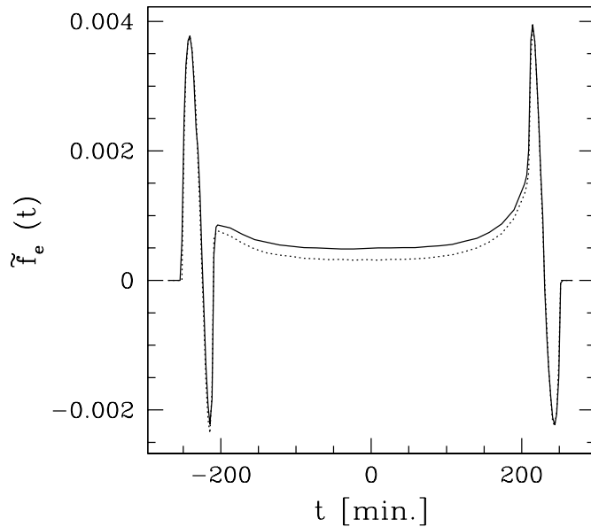
FIG. 10.—Fractional difference between the light deficit from an elliptical fiducial model and a spherical model, \tilde{f}_e (eq. [17]), with parameters of the spherical model tuned to minimize this fractional difference. The solid line is for a model with lensing, and the dotted line is for a model without lensing. The derived parameters of the spherical planet are R_0 = 35,230 km, u_* = 0.8048 , and v_* = -0.227 for the lensed case (solid line) and R_0 = 35,270 km and the same u_* and v_* for the unlensed case (dotted line). The dotted line is essentially the fractional difference in the light deficit of an elliptical compared to a spherical planet of a similar total area. See text for details.
