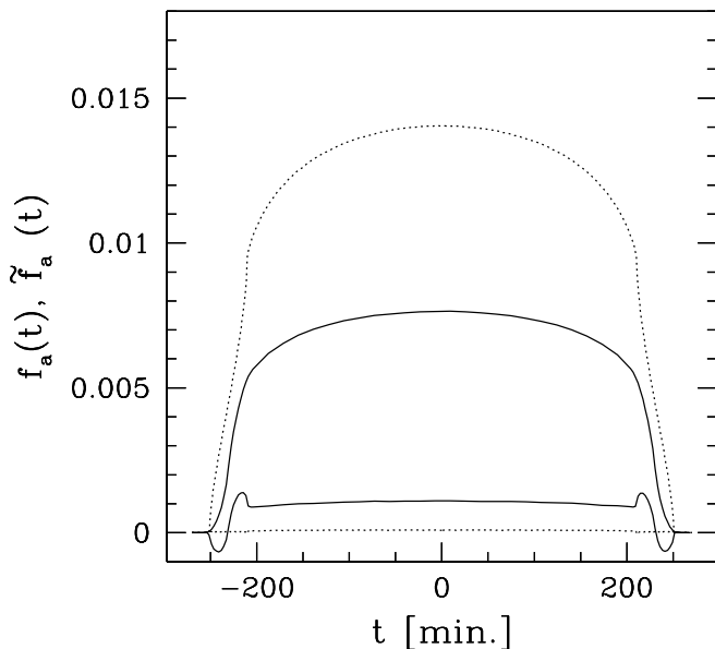
FIG. 12.—The f_a(t) (eq. [21]) for cases with and without lensing ( upper solid and dotted lines, respectively ). The lower solid and dotted lines show the corresponding \tilde{f}_a(t) (eq. [22]), which is a minimized function. The small values of the lower two lines demonstrates that an appropriate R_0 can always be chosen so that the step function model approximates a more realistic absorption model to high accuracy.
