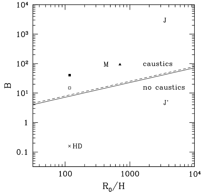
FIG. 3.—Separation of the strong lensing regime (existence of caustics) from the weak lensing regime for the combination of parameters B and R_0/H (delineated by solid and dashed lines). The solid line is for projected oblateness/ellipticity \epsilon = 0.1 , and the dashed line is for a sphere, \epsilon = 0 . The parameter B is defined as B = 2\alpha(\rho_0/H)D_{LS}D_{OL}/(D_{OL} + D_{LS}) (eq. [9]). The quantity R_0/H is the ratio of planet radius to atmospheric scale height. We show values of B and R_0/H for HD 209458b (HD), where D_{LS} \ll D_{OL} , and for Mars (M) and Jupiter (J), where D_{LS} \gg D_{OL} . In all cases, observations at optical wave bands are assumed. We show with the symbol J' the parameters for Jupiter if it were observed at wave bands with 600 times stronger absorption (e.g., in the UV; see text for details). The filled square denotes the fiducial model we study in this paper. The triangle, open square, and cross are other models we also discuss.
