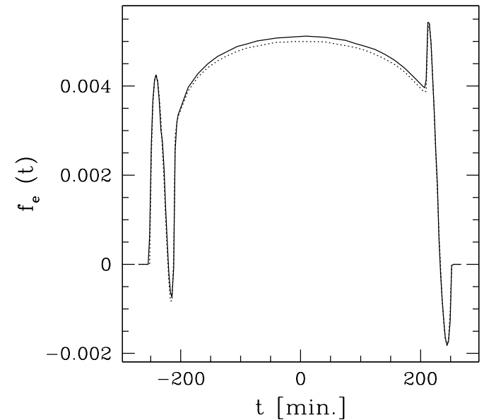
FIG. 9.—Fractional difference between the light deficit from a transit of an elliptical planet and a spherical planet, f_e , for the fiducial model denoted by the filled square in Fig. 3. The solid line is for a transit with lensing and the dotted line for a transit without.
