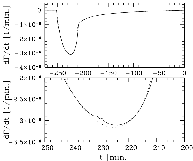
FIG. 8.—The dF/dt for the fiducial model with \epsilon = 0.05 , denoted by the filled square in Fig. 3. The lower panel is a magnified version of the upper one. The solid line is with lensing, and the dotted line is without.
