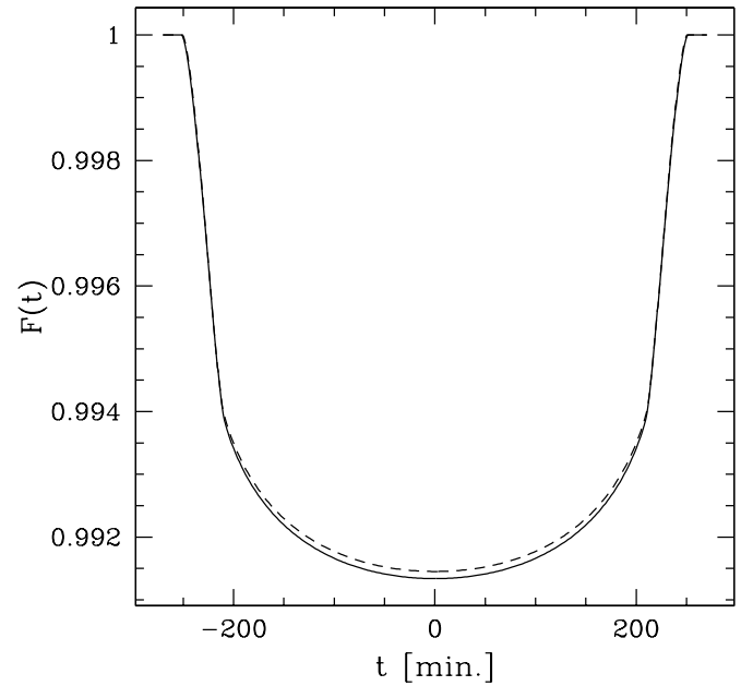
FIG. 5.—Transit light curve for our fiducial model (denoted by a filled square in Fig. 3) with atmospheric lensing ( solid curve ) and without ( dashed curve ). F(t) is the normalized stellar flux (eq. [7]). The star here has R_* = 0.6 R_\odot .
