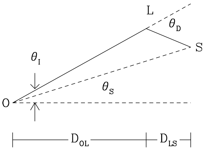
FIG. 1.—Schematic ray-tracing diagram; the solid line joining O (observer), L (lens), and S (source) represents the light ray. L represents the point of closest approach in the transiting planet's atmosphere. S represents a point on the surface of the star. The deflection is exaggerated, and the diagram is not to scale. We use the convention that \theta_D has an opposite sign to \theta_I and \theta_S .
