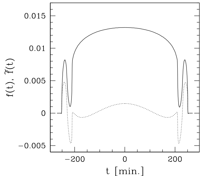
FIG. 6.—Fractional difference between the flux deficit from a stellar light curve, f(t) , with and without planetary atmospheric lensing ( solid line ; eq. [14]). This is for the fiducial model denoted by the filled square in Fig. 3. The dotted line shows \tilde{f}(t) as defined in eq. (15), the fractional difference between the light deficit from a lensed fiducial model and an unlensed model with parameters of the unlensed model tuned to minimize this fractional difference: R_0 = 35,400 km, H = 300 km, R_* = 417,600 km, u_* = 0.832 , v_* = -0.2475 , \rho_0 = 1.68 \times 10^{-5} , \epsilon = 0.05 , w = 2.9741 \times 10^{-13} s ^{-1} , \gamma_{\text{tr imp}} = 49^\circ 5 , and \theta_{\text{tr imp}} = 69,696 km/ D_{OL} .
