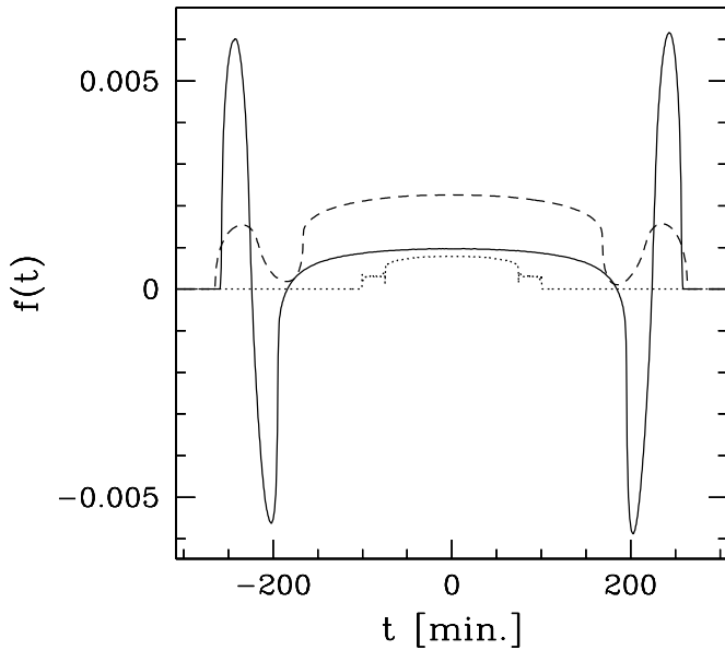
FIG. 7.—The f(t) (eq. [14]) for three different planetary models corresponding to the open square (solid line), cross (dotted line), and triangle (dashed line) in Fig. 3. Parameters for the dotted line resemble those for HD 209458b.
