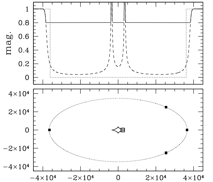
FIG. 4.— Top : Magnification as a function of source position for source positions (dashed line; overlaps with solid line in the upper portion) that lie on the major axis of the planet (the x -axis in the lower panel). The dotted line shows the occultation kernel W as defined in eq. (8). The solid line represents the light curve for an occultation by a solar system planet of a distant star, which happens to be moving along the planet's semimajor axis. See text for details. Bottom : Caustic, source positions where the magnification diverges (solid line), while the dotted line shows the critical curve, which is the image of the caustic. The four filled squares are images of a point source denoted by an open square situated just inside the caustic. The axis coordinates are distances (in kilometers) in the lens plane; i.e., they correspond to physical distances from the planet center.
