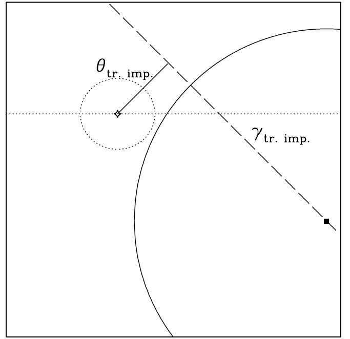
Fig. 2.—Geometrical set up of a planetary transit. The circular solid line represents the boundary of the star, while the ellipsoidal dotted line represents that of the planet. The filled square is the center of the star, which moves along the dashed line with respect to the planet. The horizontal dotted line defines the major axis of the planet; \gamma_{\text{tr imp}} is the angle between the horizontal and dashed line, while \theta_{\text{tr imp}} is the distance in angular units of closest approach between the planet center and the stellar center.
