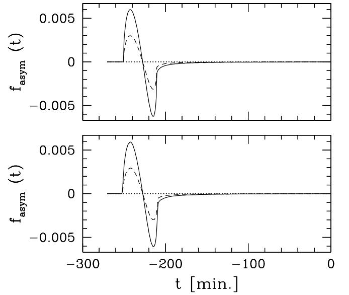
FIG. 11.—Value of f_{\text{asym}} as defined in eq. (18) with (bottom) and without (top) lensing. The solid line is for \epsilon = 0.1 , the dashed line is for \epsilon = 0.05 , and both are for \gamma_{\text{tr imp}} = 45^\circ . The dotted line is for the same \epsilon but with \gamma_{\text{tr imp}} = 0^\circ . In all cases, the rest of the parameters are those of the fiducial model (filled square in Fig. 3). If the curves in the upper and lower panels are plotted together, they almost completely overlap; i.e., light curves with and without lensing have an almost identical degree of oblateness-induced asymmetry.
