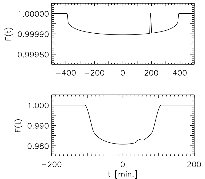
FIG. 13.—Effect of a planet crossing an Earth-sized star spot on a stellar disk. Top : An Earth-like planet transit. Bottom : A close-in EGP-like planet transit.
