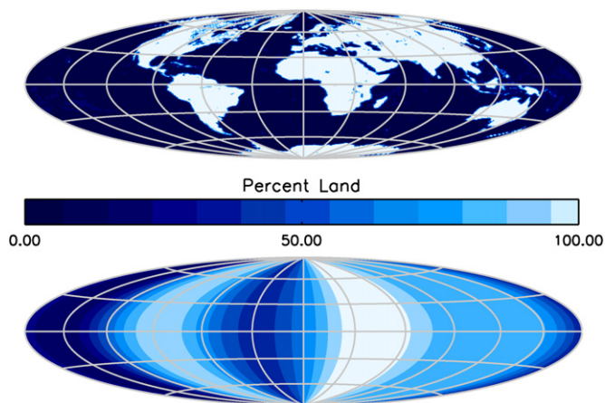
Figure 10. Aitoff projection showing the land distribution on Earth in a cloud-free MODIS map (top panel) and the distribution of land as determined from the June disc-integrated EPOXI light curves (bottom panel). The EPOXI map has a longitudinal resolution of approximately 60^\circ ; it has no latitudinal resolution, but is weighted toward the equator due to viewing geometry.
