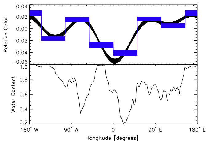
Figure 8. Comparison of N -slice (blue) and sinusoidal (black) longitudinal maps of the blue eigencolor based on the March EPOXI observations (top panel) to the MODIS cloud-free, equator-weighted distribution of oceans (bottom panel). The thickness of the lines in the top panel shows the 1\sigma uncertainty on the maps. The fit to Earth's latitudinally averaged water content is not excellent, noticeably the Atlantic Ocean and the Americas. The discrepancy is due to cloud cover, as discussed in the text.
