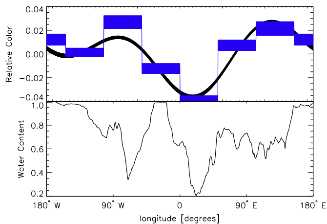
Figure 9. Comparison of N -slice (blue) and sinusoidal (black) longitudinal maps of the blue eigencolor based on the June EPOXI observations (top panel) to the MODIS cloud-free, equator-weighted distribution of oceans (bottom panel). The thickness of the lines in the top panel shows the 1\sigma uncertainty on the maps. The fit to Earth's latitudinally averaged water content is not excellent, noticeably the Atlantic Ocean and the Americas. The discrepancy is due to cloud cover, as discussed in the text.
