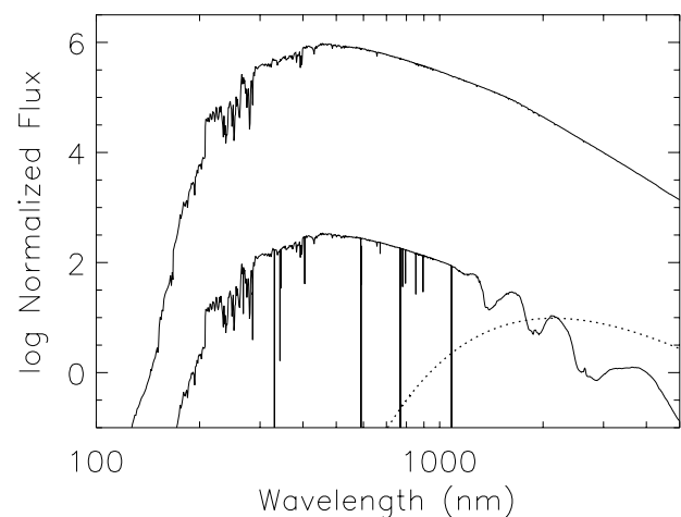
FIG. 1.—Flux of HD 209458 a ( upper curve ) and the transmitted flux through the planet's transparent atmosphere ( lower curve ). Superimposed on the transmitted flux are the planetary absorption features, including the He I triplet line at 1083 nm. The other bound-bound lines are alkali metal lines (see Fig. 2 for details). The \text{H}_2\text{O} and \text{CH}_4 molecular absorption dominates in the infrared. The dotted line is a blackbody of 1350 K representative of the CEGP's thermal emission, but the thermal emission can be larger than a blackbody blueward of 2000 nm.
