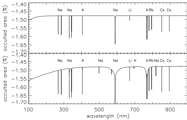
FIG. 2.— Upper plot : The normalized in-transit minus out-of-transit spectra, i.e., percent occulted area of the star. In this model the cloud base is at 2.4 \times 10^{-3} bar. Rayleigh scattering is important in the UV. Lower plot : A model with cloud base at 0.2 bar. The stellar flux passes through higher pressures, densities, and temperatures of the planet atmosphere compared to the model in the upper plot. In addition, a larger transparent atmosphere makes the line depth larger. Observations will constrain the cloud depth. See text for discussion.
